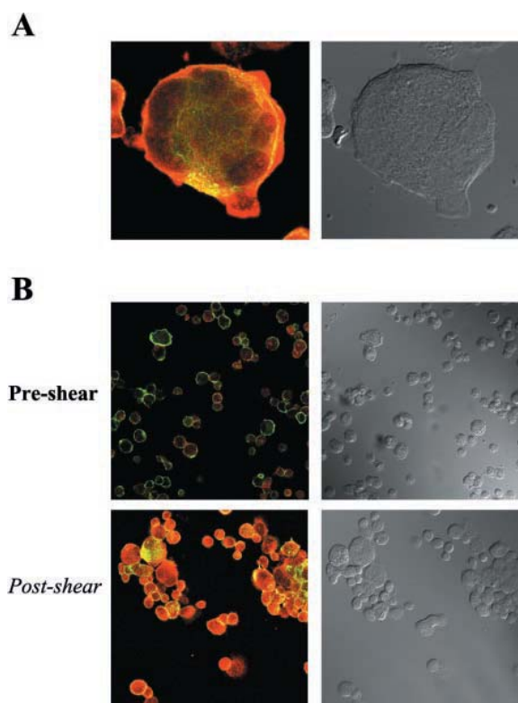
Fig. 8. Shear augmented the expression of \alpha_v\beta_3 in tumor cells. We investigated the clustering effect of \alpha_v\beta_3 in tumor cells pre- and postshear. A : RBM/E-3 cells were exposed to a continuous shear rate of 400\text{ s}^{-1} and then stained with anti- \alpha_v\beta_3 . B : distinct differences between sheared and non-sheared cells were observed, with sheared cells showing a significant increase in staining intensity.
