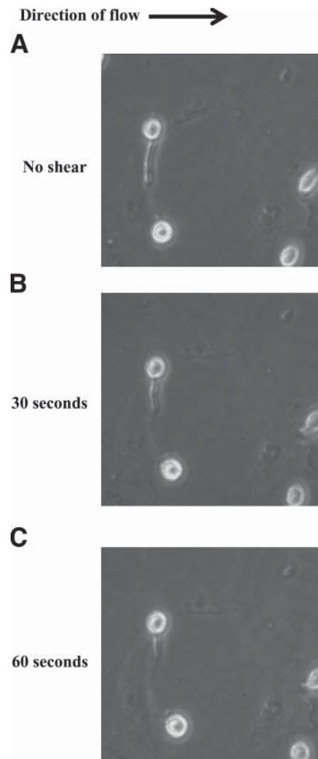
Fig. 3. The morphological response of HuT cells under shear stress is different in malignant cells. HuT cells were perfused across LPS-stimulated HUVECs. Between shear rates of 0 and 100 \text{ s}^{-1} , a long, single pseudopodal structure formed (A, no shear). At a shear rate of 200 \text{ s}^{-1} , rapid retraction of the tail occurred over a 1-min period (B, 30 s, C, 60 s).
