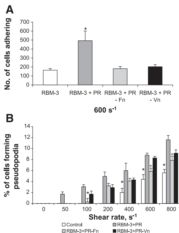
Fig. 7. Secreted platelet Vn and Fn contribute to tumor cell arrest at high venous shear rates. The immunodepleted releasates were preincubated with RBM/E-3 cells before flow. A: at venous shear rates of 600 and 800 s^{-1} , a significant decrease in tumor cell adhesion was detected ( *P < 0.0001 compared with RBM-3 + PR). Results in B represent pseudopod formation at all shear rates. Less pseudopod formation was observed with immunodepleted Fn releasates than with immunodepleted Vn releasates ( +P < 0.0033 ).
