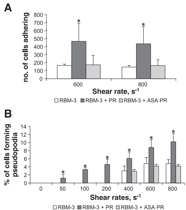
Fig. 1. Adhesion and shear-induced activation are enhanced by platelet releasate. Aspirin [acetylsalicylic acid (ASA)] abrogates the enhanced effects of platelet releasate (PR). RBM/E-3 cells were perfused across LPS-stimulated human umbilical vein endothelial cells (HUVECs) at incremental shear rates from 50 to 800 \text{ s}^{-1} . The results shown in A represent the average number of untreated and PR-treated cells adhering at shear rates of 600 and 800 \text{ s}^{-1} . There was significant increase in the number of PR-treated cells (RBM-3 + PR) adhering to HUVECs compared with untreated cells (RBM-3) or aspirin-PR-treated cells (RBM-3 + ASA PR) ( *P < 0.001 ). B : percentages of cells actively forming pseudopodia at incremental shear rates ( n = 10 ). RBM/E-3 cells activated at significantly lower shear rates in the presence of PR ( *P = 0.003, n = 6 ), and this effect was abolished by aspirin treatment.
