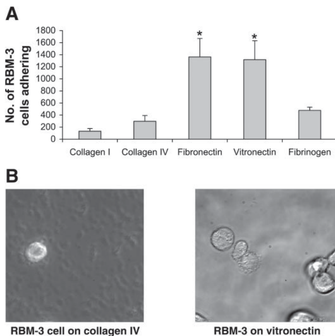
Fig. 4. RBM/E-3 cells adhere and activate more on vitronectin (Vn) and fibronectin (Fn) than on other extracellular matrices. The cells were exposed to a continuous shear rate of 100, 200, or 400 s^{-1} for 1 h. Results shown in A represent the number of adherent RBM/E-3 cells after a continuous shear rate of 100 s^{-1} . Maximal adhesion occurred on Vn and Fn, with nearly 3 times the number of RBM/E-3 cells adhering, compared with collagen (types I and IV) and fibrinogen ( P < 0.0001 ). B : different morphological responses of different matrix proteins are demonstrated by the RBM/E-3 cells on collagen IV ( left ) and Vn ( right ). The formation of pseudopodia and spreading were not evident on collagen IV; however, on Vn, rapid formation of pseudopodia preceded spreading within minutes.
