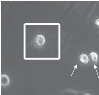
Fig. 2. RBM/E-3 cells activate in response to a shear rate of 400 \text{ s}^{-1} . At a shear rate of 400 \text{ s}^{-1} , a rapid morphological response occurred wherein 3% of adhering RBM/E-3 cells rapidly extended and retracted pseudopodia within 200 ms over the surface of the cell. A representative activated cell is shown within box at center. Quiescent cells are present at right and are indicated by arrows. Please refer to the Supplementary Material for this article (published online at the American Journal of Physiology-Cell Physiology web site) to view Movies 1–3.
