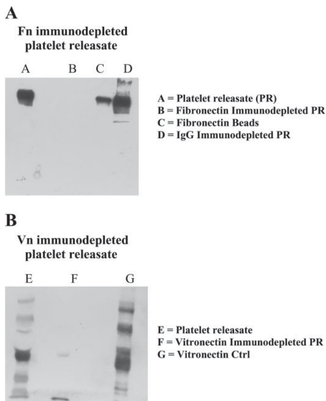
Fig. 6. Immunodepletion of Fn and Vn from platelet releasate. The physiological importance of platelet-secreted Vn and Fn in tumor activation was further examined. Western blot analysis confirmed the presence of Vn and Fn in platelet releasate and their corresponding depletion from platelet releasates (A and B).
