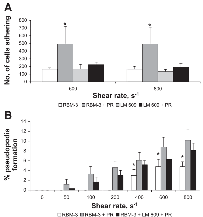
Fig. 5. Monoclonal antibody anti- \alpha_v\beta_3 inhibits PR-induced cell adhesion and activation to HUVECs under shear conditions. Blocking \alpha_v\beta_3 alone in RBM/E-3 cells results in less adhesion at shear rates of 50–800 s^{-1} . A : pretreatment of RBM/E-3 cells with anti- \alpha_v\beta_3 antibody LM609 significantly reduced the potentiating effect of PR on RBM/E-3 cell adhesion to HUVECs under shear conditions. The number of adherent cells decreased 2-fold compared with PR-treated cells ( *P < 0.001 ) to levels similar to those for untreated cells or cells treated with LM609 alone. B : a decrease in pseudopod formation was observed when PR-treated cells were preincubated with \alpha_v\beta_3 antibody. However, this was not significant ( P = 0.4711 ). At all shear rates, pseudopod formation was significantly lower in untreated RBM/E-3 cells compared with PR- and LM609 + PR-treated cells ( *P < 0.001 ).
