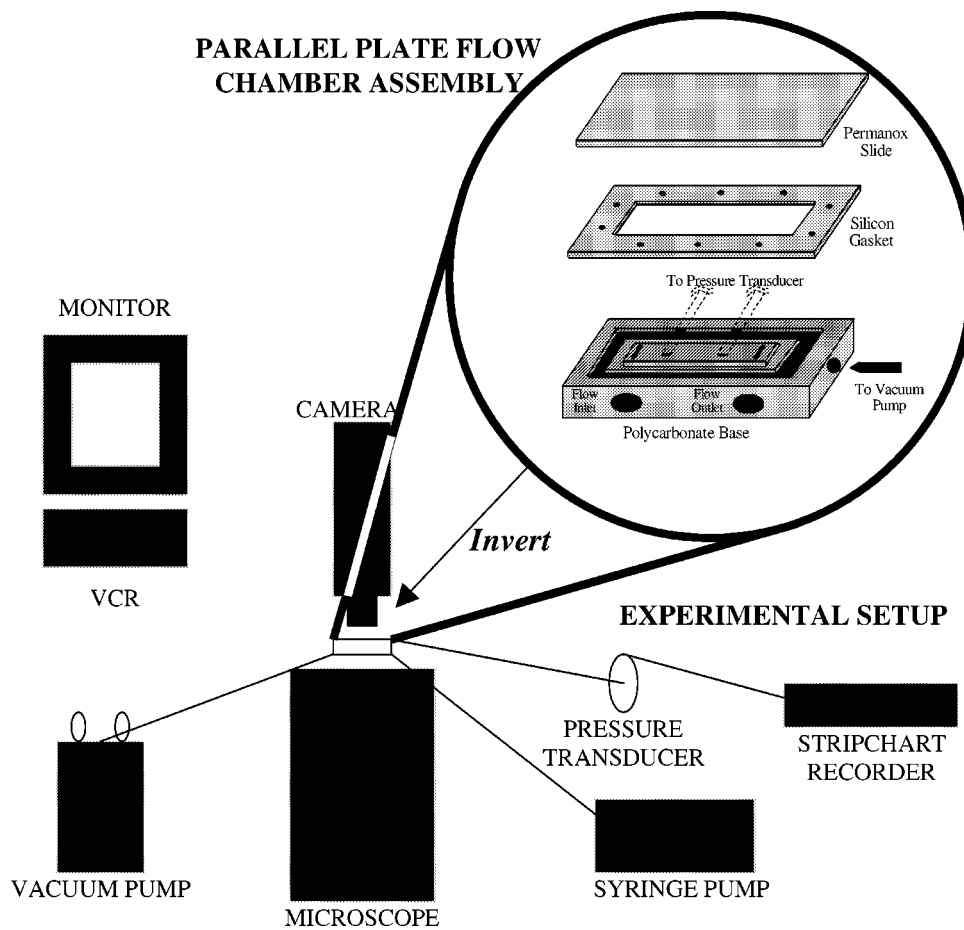
Fig. 1. Schematic of experiment setup employed in the detachment assay. The parallel plate flow chamber is inverted on the microscope stage such that the endothelial monolayer composes the bottom of the chamber.
