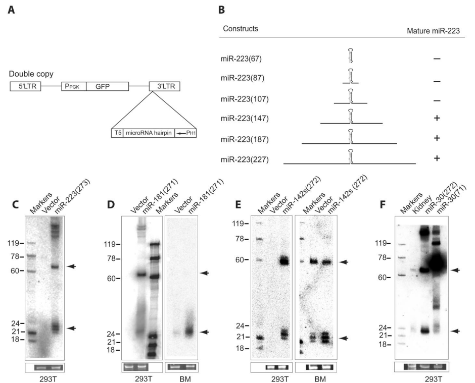
Fig. 3. A general strategy for the ectopic expression of miRNAs. (A) The retroviral construct for miRNA expression. A pol III expression cassette containing the human H1 promoter (P H1 ), the miRNA hairpin, and the T5 termination signal was placed in the U3 region of the viral 3' long terminal repeat (LTR). As a marker for infection, the vector also expressed the gene for GFP under control of the constitutive murine 3-phosphoglycerate kinase promoter (P PGK ). This vector configuration, which improves stable gene expression in primary cells, was termed "double copy," because the process of retroviral reverse transcription and integration causes two copies of the miRNA expression cassette to be integrated into the host genome (29). (B) Summary of miR-223 expression and maturation from vectors designed to express successively longer miR-223 genomic fragments, each containing the miR-223 predicted hairpin and flanking sequences. miR-223(67), (87), (107), (147), (187), and (227) transcripts included the 67-nt miR-223 predicted hairpin at their center, with 0, 10, 20, 40, 60, or 80 nt of genomic sequence flanking each side of the hairpin, respectively. Expression and maturation of miR-223 in transfected 293T cells was examined by Northern analysis. High expression of the primary transcript was seen for each of the three constructs that did not generate mature miRNA. (C to E) Expression of miR-223, miR-181, and miR-142s from ~270-nt primary transcripts that included the ~22-nt mature miRNA and 125 nt of genomic sequence flanking each side of the miRNA, in transfected 293T cells or viral-transduced mouse bone marrow cells (BM). (F) Expression of miR-30 from the 71-nt predicted miR-30 hairpin or a 272-nt fragment with 125 nt of genomic sequence flanking each side of the miRNA. Ethidium staining of 5S ribosomal RNA served as the loading control.
